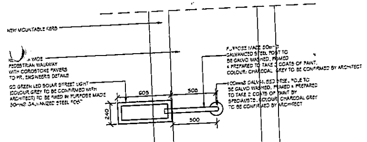
STEEL POST DETAIL SCALE: 1: 20
